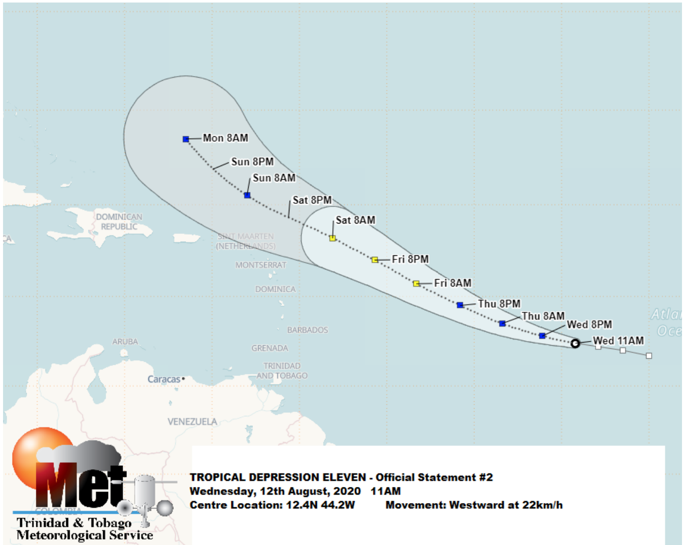
Figure 1. Forecast track of Tropical Depression Eleven
